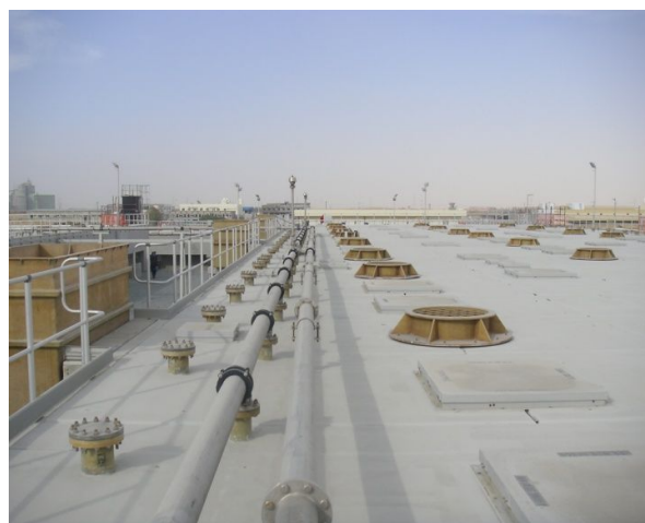
Gas Piping System in UASB Reactor
